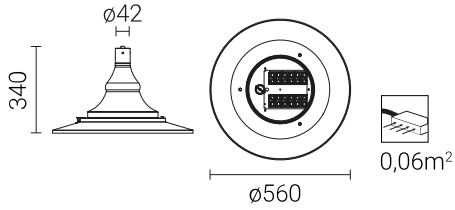
OW+ LED D4i WITH DIFFUSER
