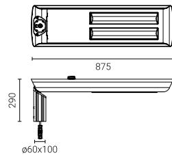
CUDDLE II LED REG D4i x2 96W, 120W, 144W, 192W
