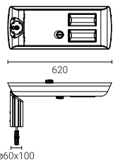
CUDDLE II LED REG D4i D 48W, 60W, 72W
