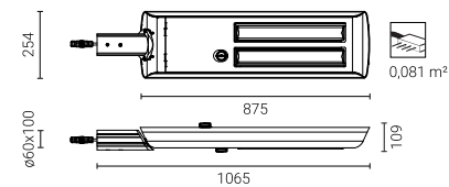
CUDDLE II LED REG D4i x2 96W, 120W, 144W, 192W
