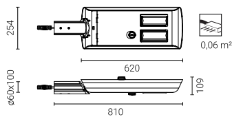
CUDDLE II LED REG x2 D4i 48W, 60W, 72W
