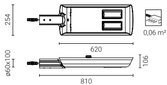
CUDDLE II LED REG D4i 48W, 60W, 72W
