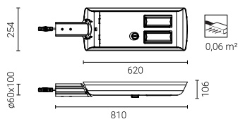
CUDDLE II LED REG D4i D 48W, 60W, 72W
