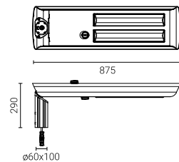
CUDDLE II LED REG D4i D 96W, 120W, 144W, 192W
