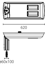
CUDDLE II LED REG x2 D4i 48W, 60W, 72W
