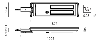
CUDDLE II LED REG D4i D 96W, 120W, 144W, 192W
