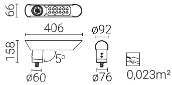
P - ISKRA LED P
